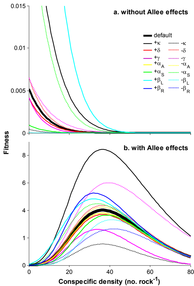
Figure S1. Sensitivity analysis of fitness models (a) without Allee effects and (b) with Allee effects. This figure illustrates the changes in the fitness model with a 20% increase or decrease in the value of each parameter (see Table 3 for parameter definitions). The thick, black line displays the default values and is the same as the thick line in Figure 2b. Note that \beta_R appears only in panel (b) because this parameter is only in the model with Allee effects (Equation 4) and that \pm\alpha_A is hidden by the default parameter line in panel (a).
